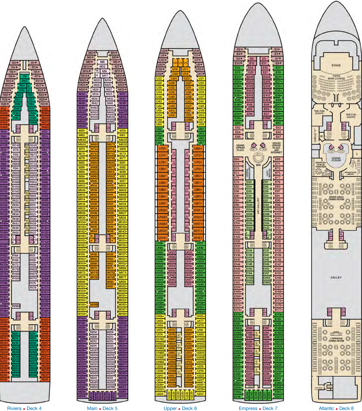
Riviera • Deck 4 Main • Deck 5 Upper • Deck 6 Empress • Deck 7 Atlantic • Deck 8
